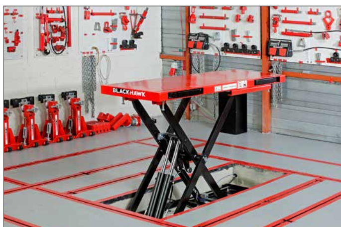
Telescopic arms
