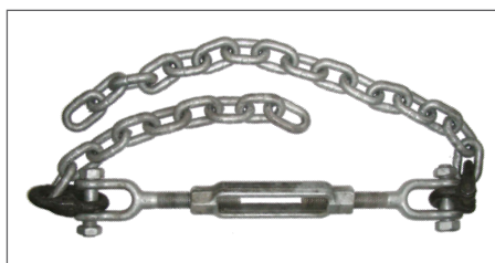
HD8302 Chain tensioner HD, chain 20 t, hook 10 t
