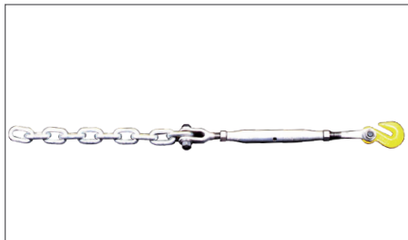
HD8302 Chain tensioner HD, chain 20 t, hook 10 t
